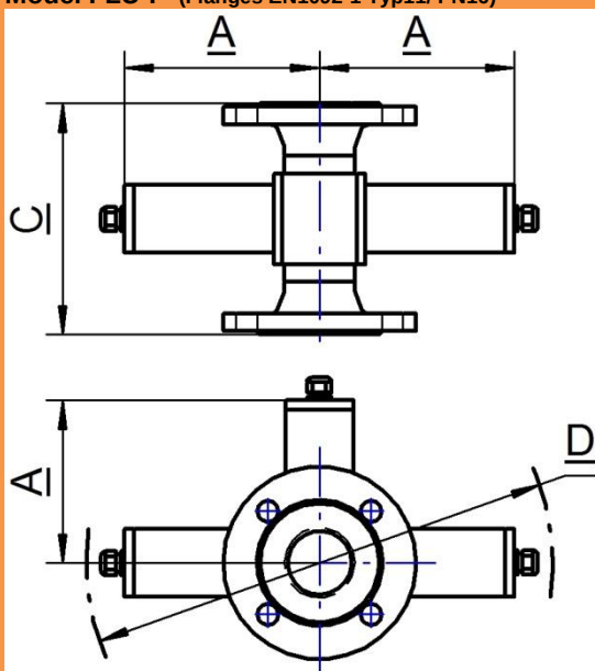
Model FLU-I (Flanges EN1092-1 Typ11/ PN16)
